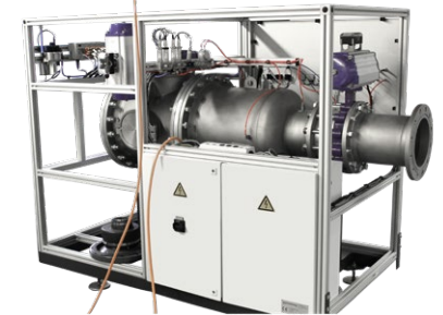
up to 18 sonic nozzle SMF®10,000
