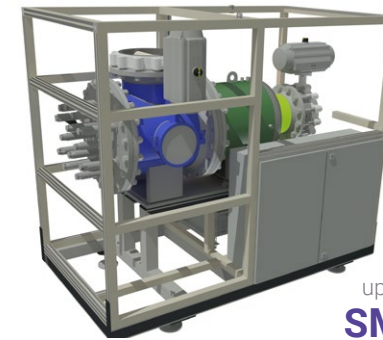
up to 9 sonic nozzle SMF®2000
